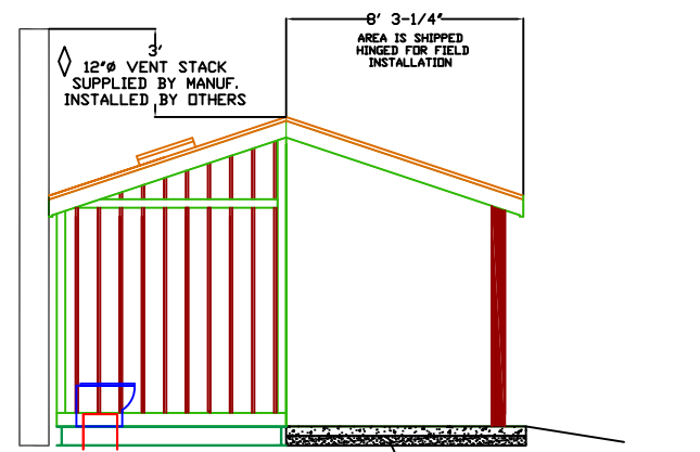
EXTENDED ROOF KIT LEFT ELEV.
