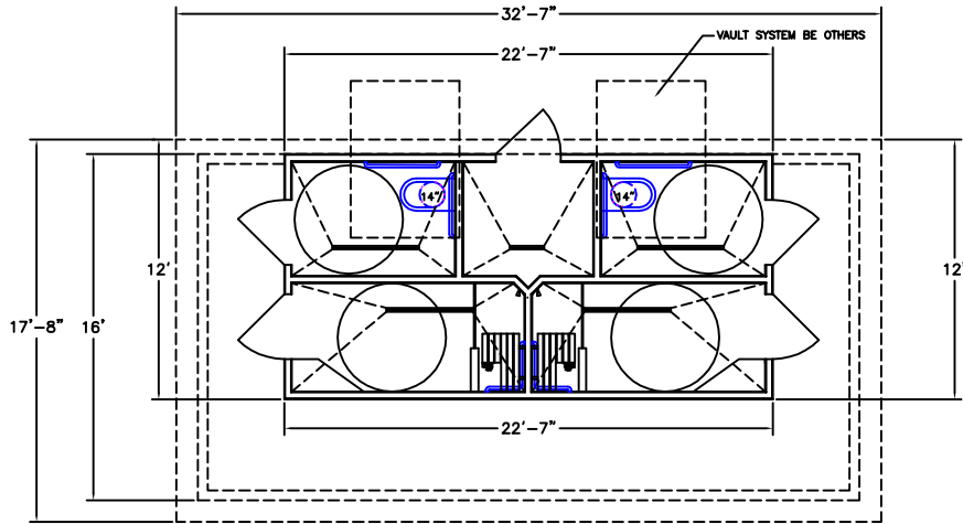
FLOOR PLAN
