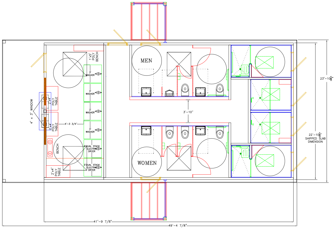
FLOOR PLAN
