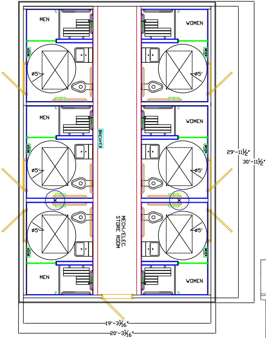
FLOOR PLAN
