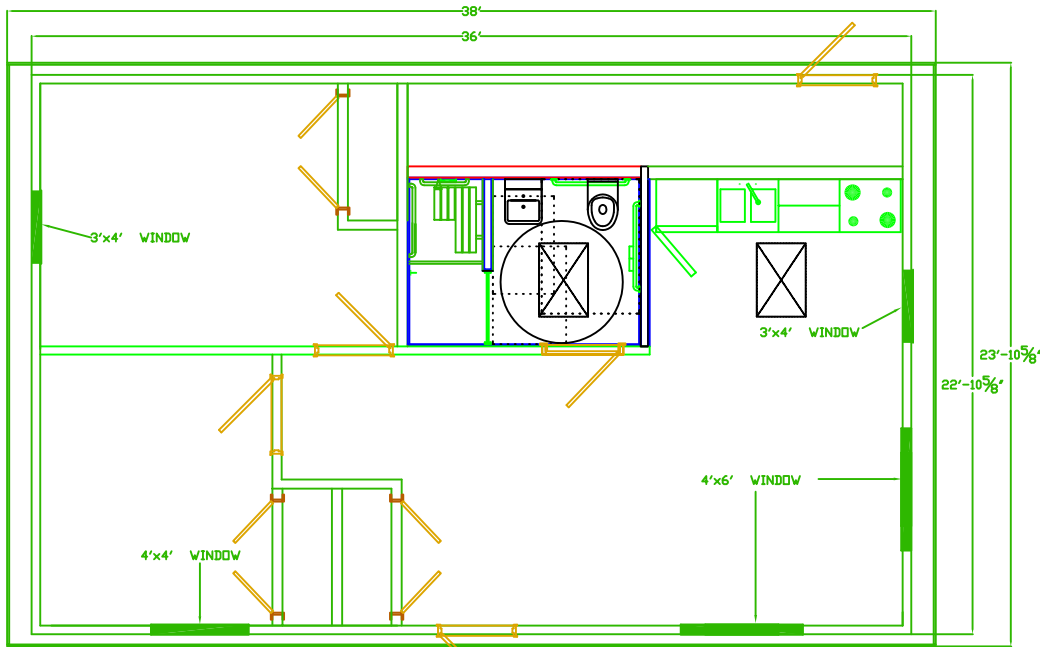
FLOOR PLAN
