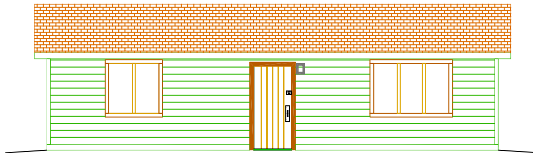
FRONT ELEVATION
