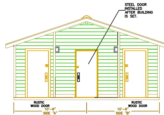
BACK ELEVATION
