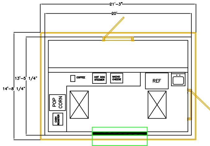
FLOOR PLAN
