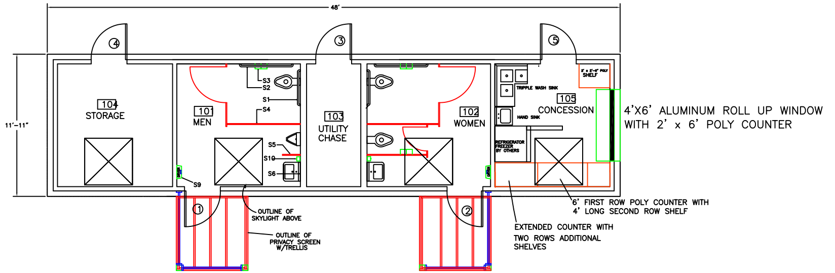
FLOOR PLAN
