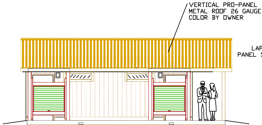
SIDE ELEVATION @ RESTROOM DOOR
