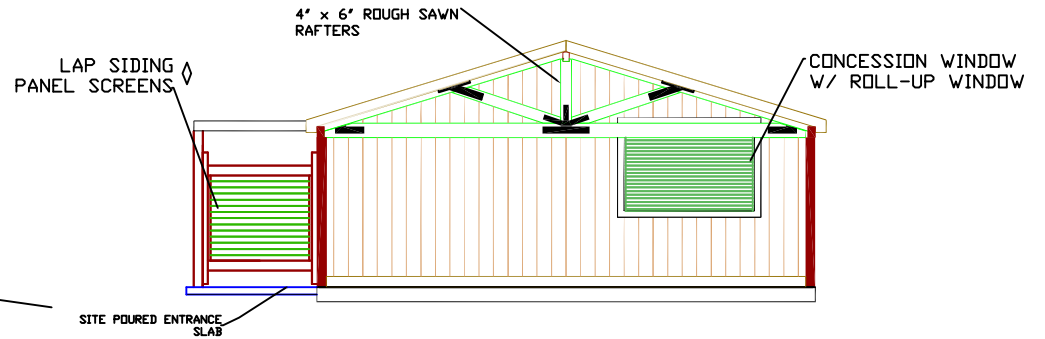
END ELEVATION @ CONCESSION WINDOW
